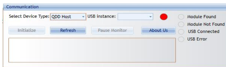
Figure 2: Communication Tab
